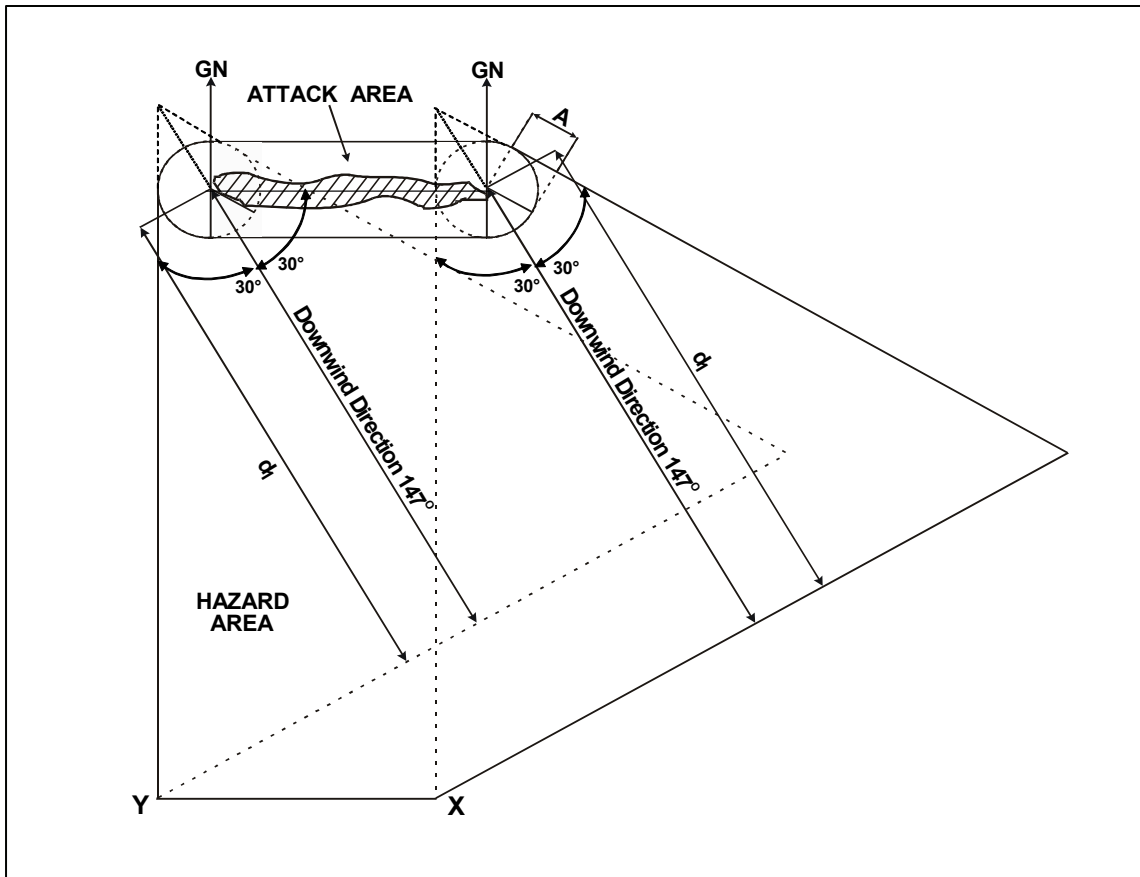
Figure F-9. Type R, Case 2, Attack
