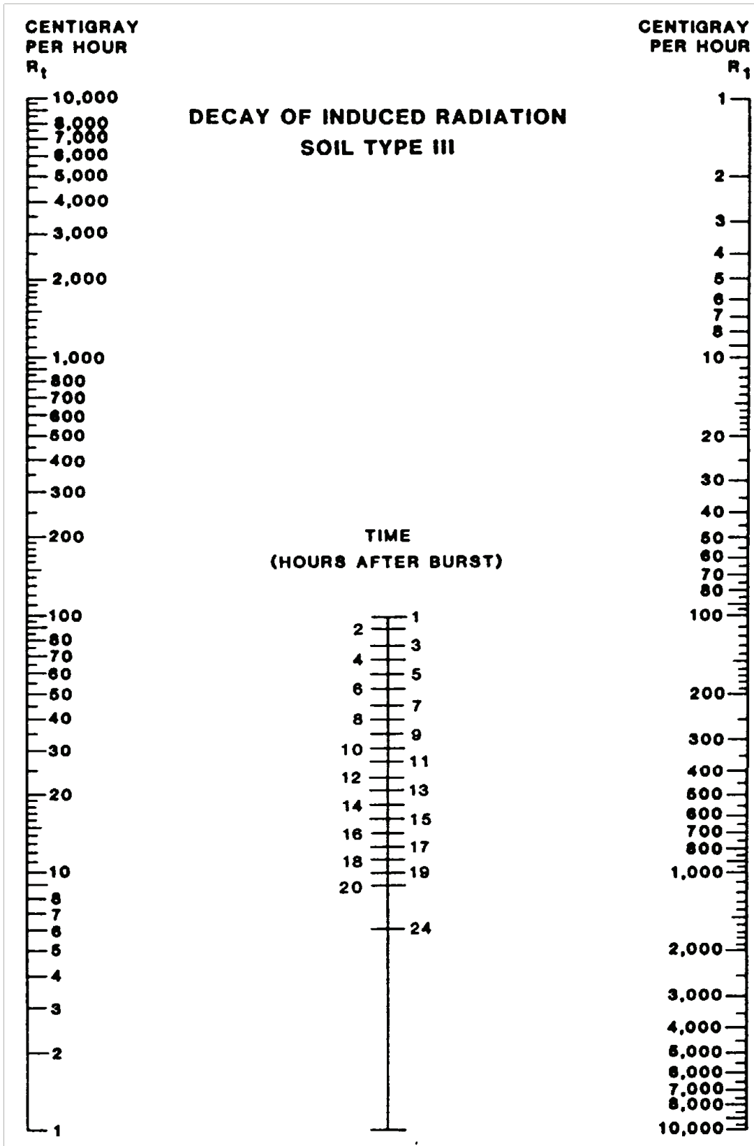
Figure J-52. Decay of Induced Radiation (Soil Type III)
