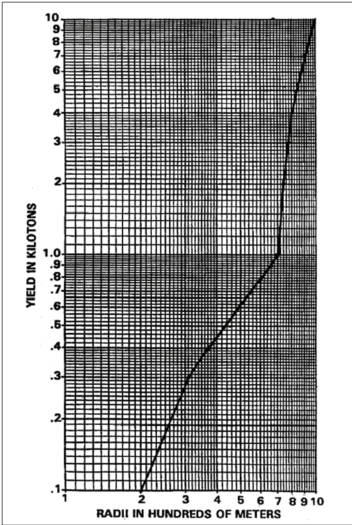
Figure G-39. Keller Nomogram for Neutron-Induced Areas From 0.1 to 10 Kilotons
