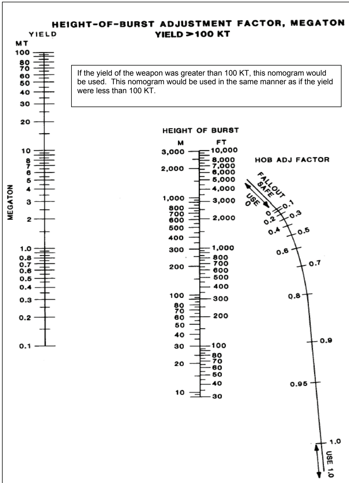
Figure G-25. HOB (Megaton) Adjustment Factor (Example)
