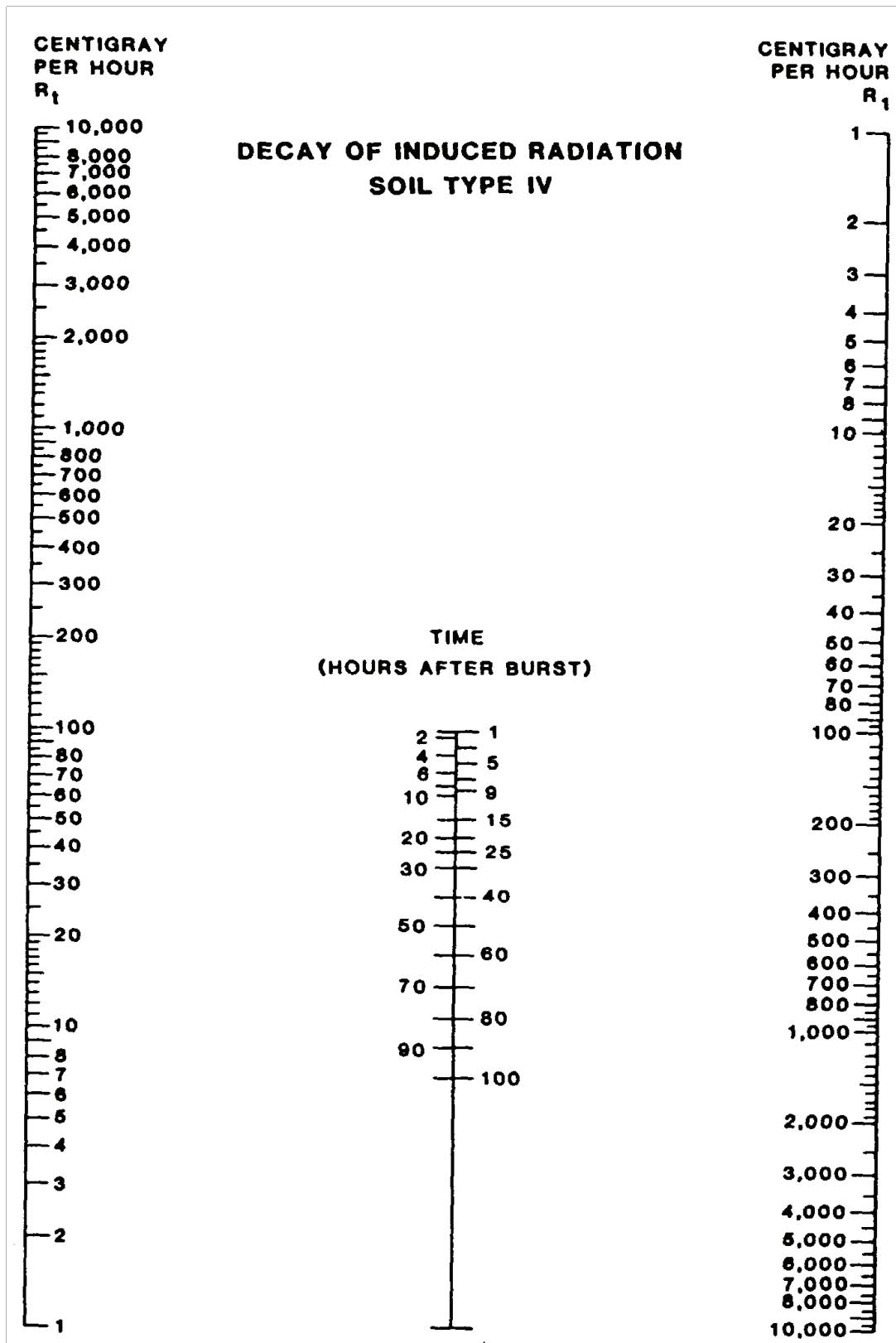
Figure J-53. Decay of Induced Radiation (Soil Type IV)
