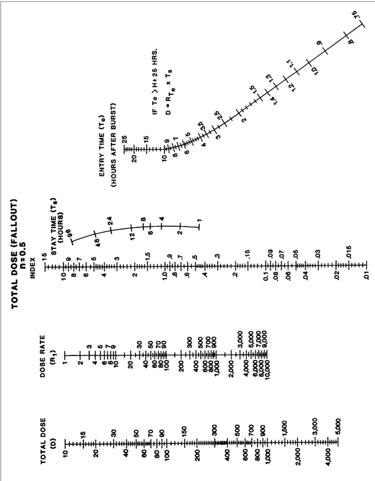
Figure J-31. Total Dose (Fallout) (n=0.5)
