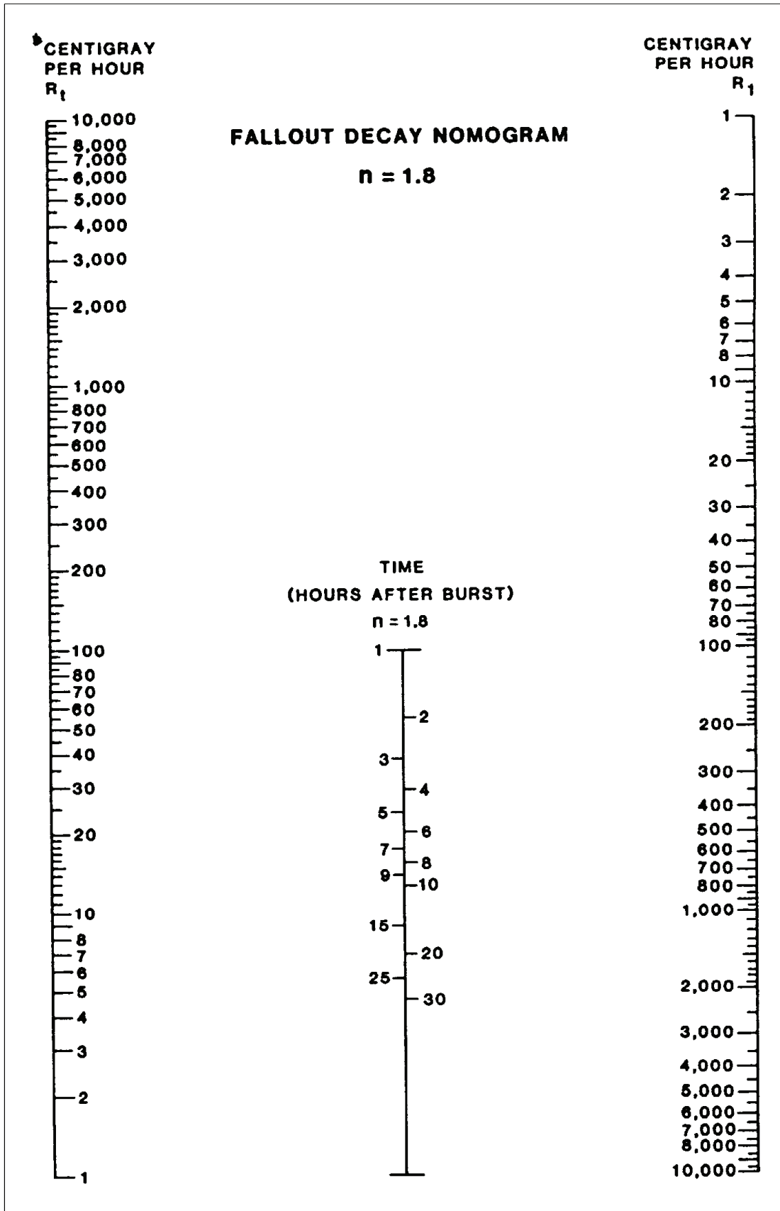
Figure J-25. Fallout Decay Nomogram ( n=1.8 )
