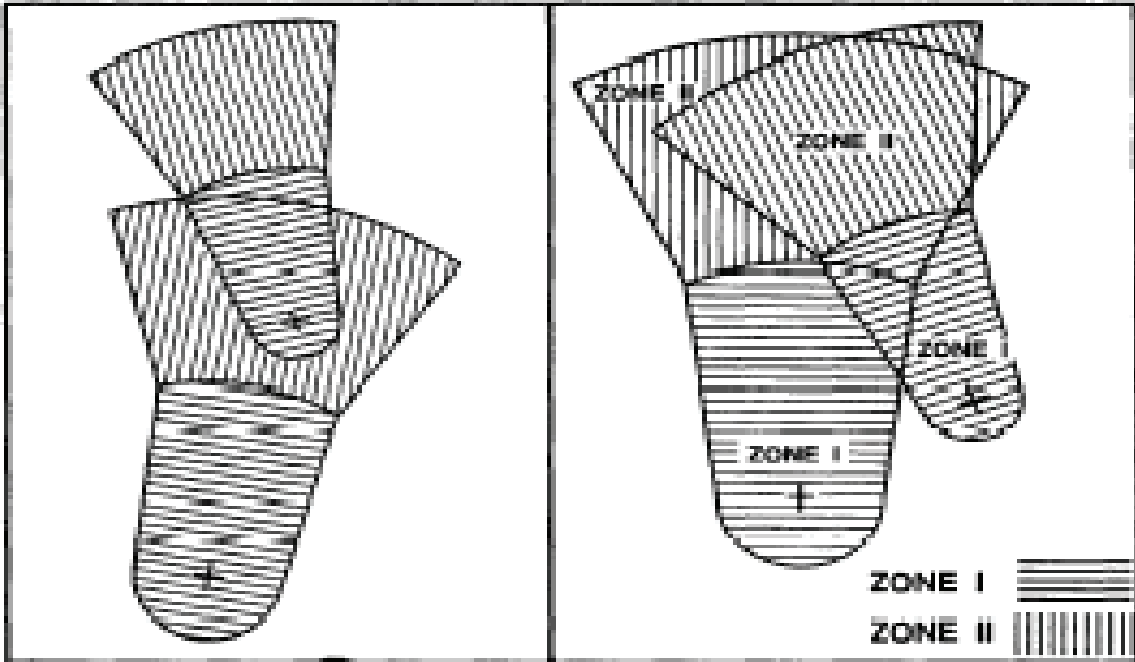
Figure G-12. Multiple-Burst Detailed Fallout Prediction (Example)
