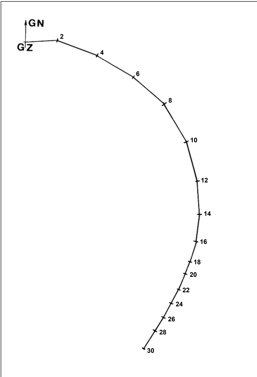
Figure D-1. Example Wind Vector Plot
