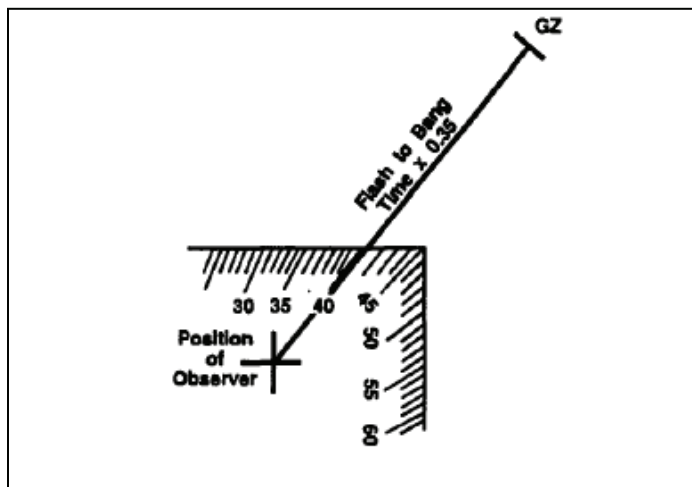
Figure G-7. Polar Plot Method
