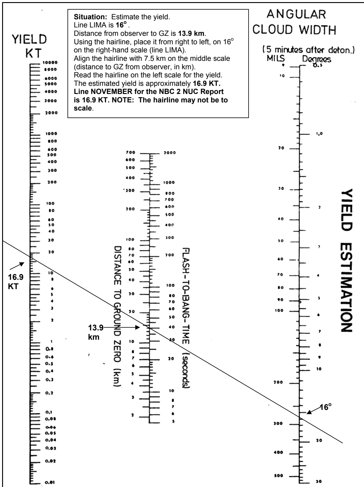
Figure G-8. Yield Estimation, Cloud Width and Flash-to-Bang Time/Distance to GZ (Example)
