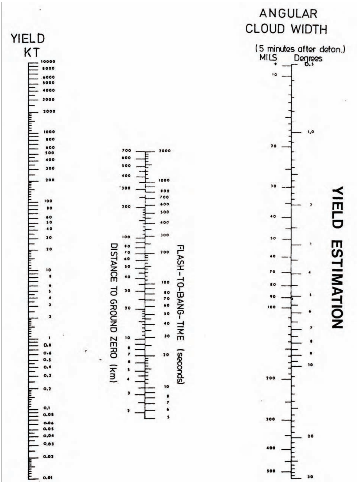
Figure J-6. Yield Estimation, Angular Cloud Width and Flash-to-Bang Time/Distance to GZ
