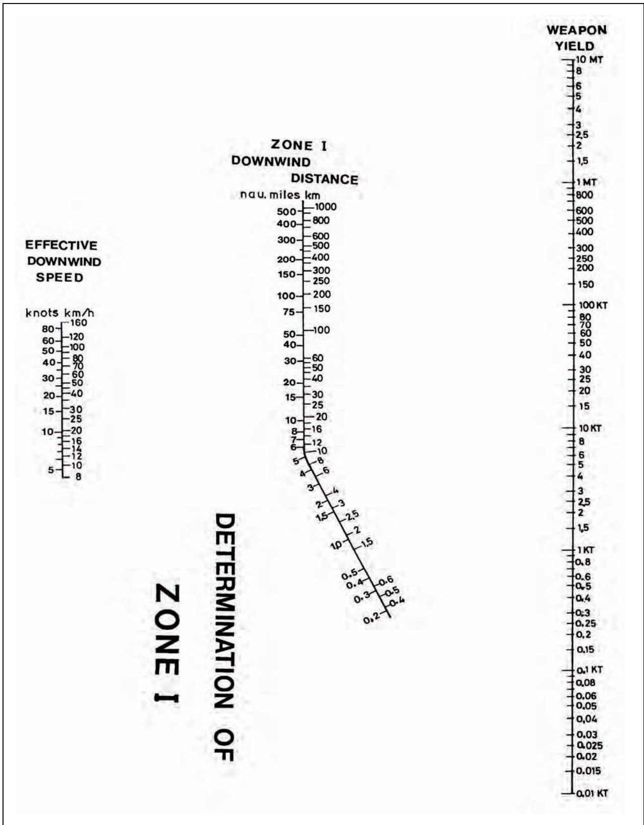
Figure G-22. Determination of Zone I, Downwind Distance (Example)
