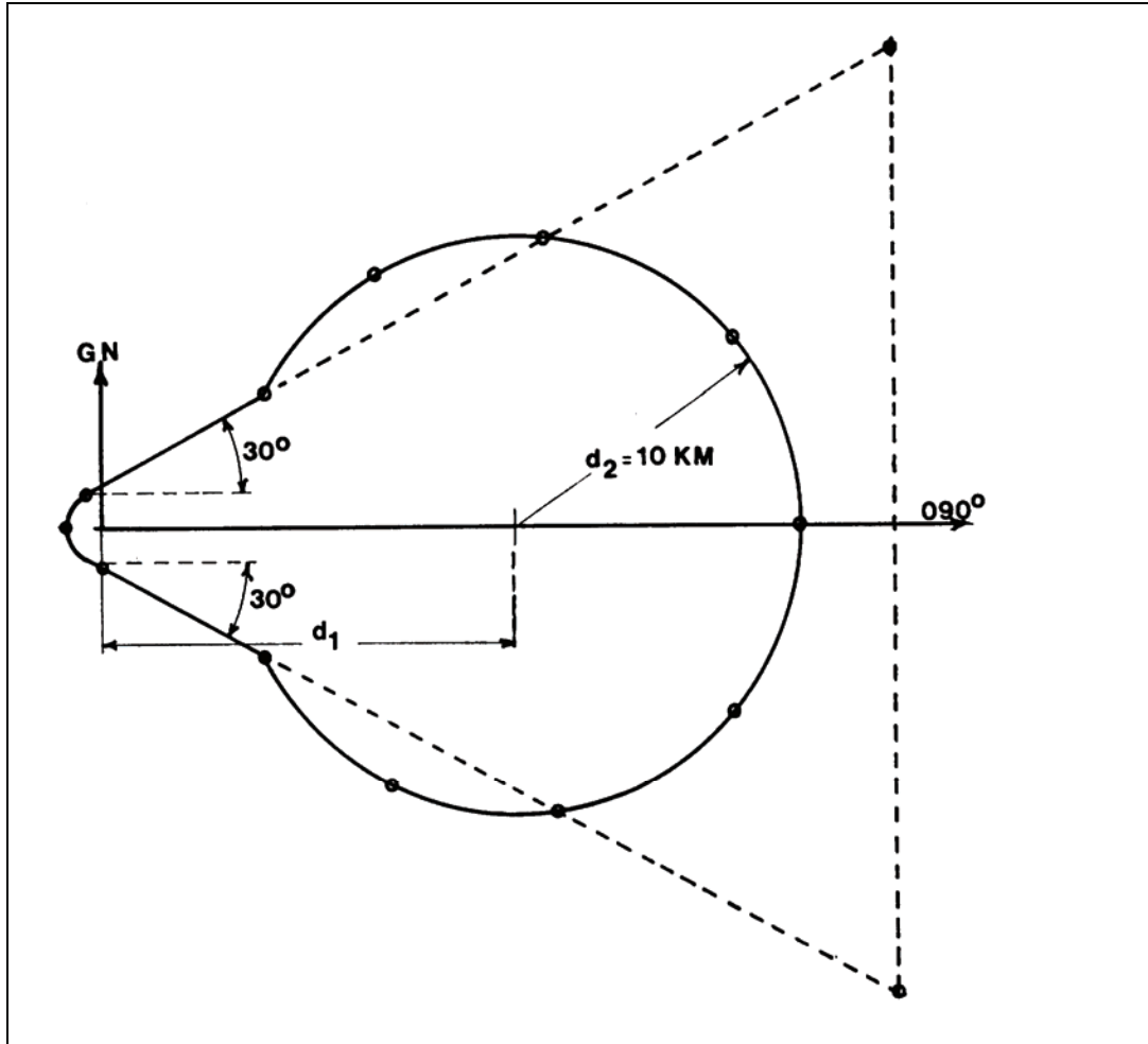
Figure E-15. Recalculation of Downwind Hazard Area Type A Attack (Change in Wind Speed From >10 kph to ≤10 kph) (Example 1)
