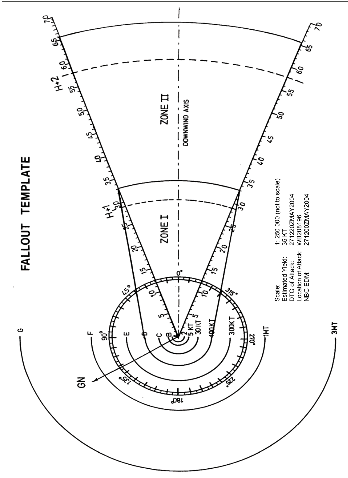
Figure G-13. Simplified Fallout Template With Fallout Prediction
