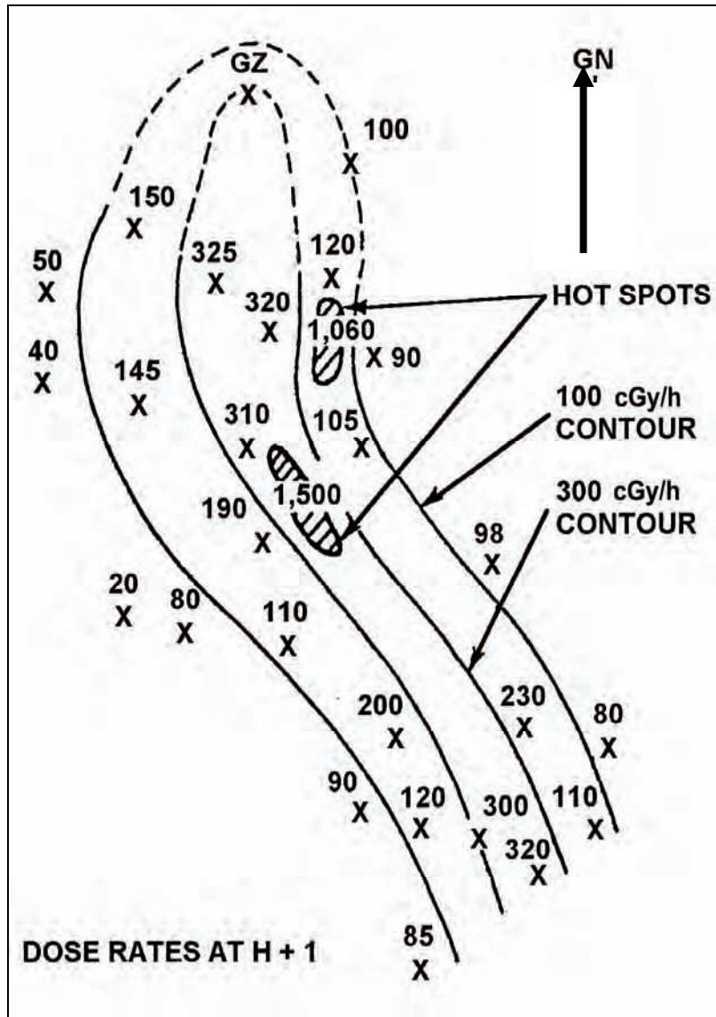
Figure G-33. Sample Fallout Pattern Plotted From Survey Data
