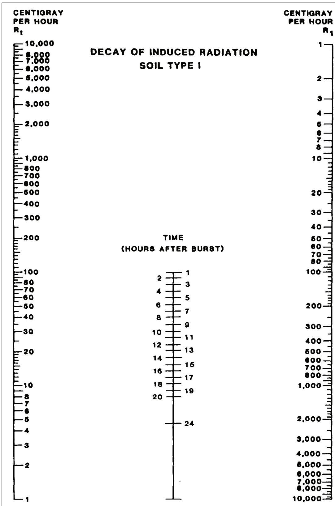
Figure J-50. Decay of Induced Radiation (Soil Type I)
