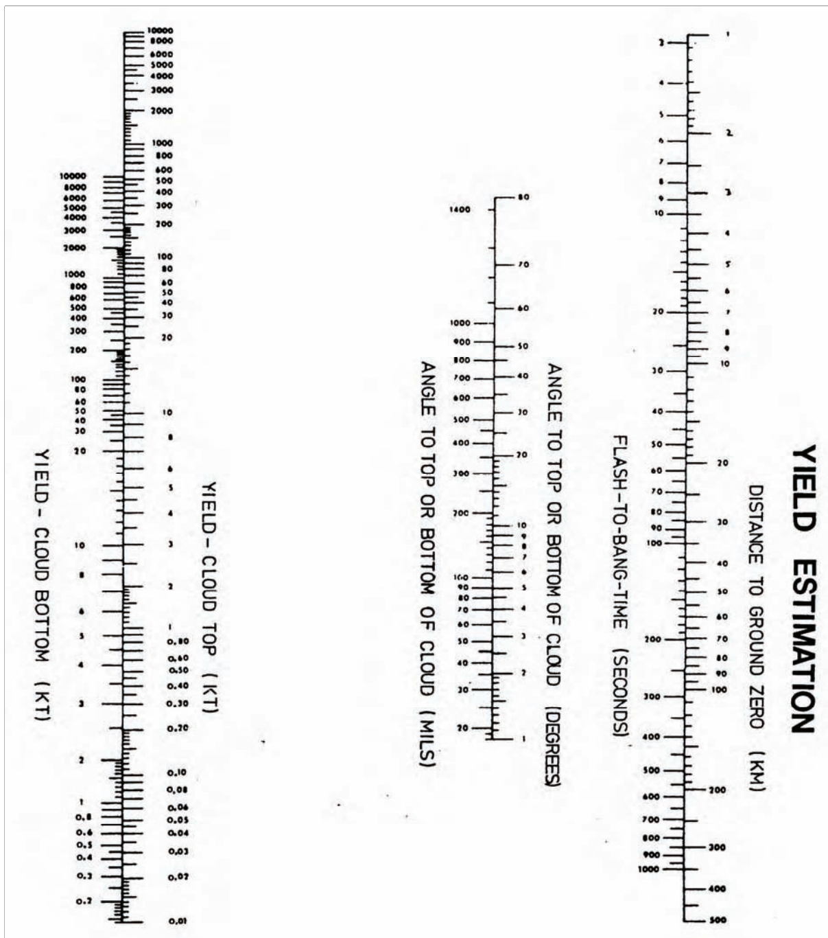
Figure J-7. Yield Estimation, Angle to Top/Bottom of Cloud and Flash-to-Bang Time/Distance to GZ
