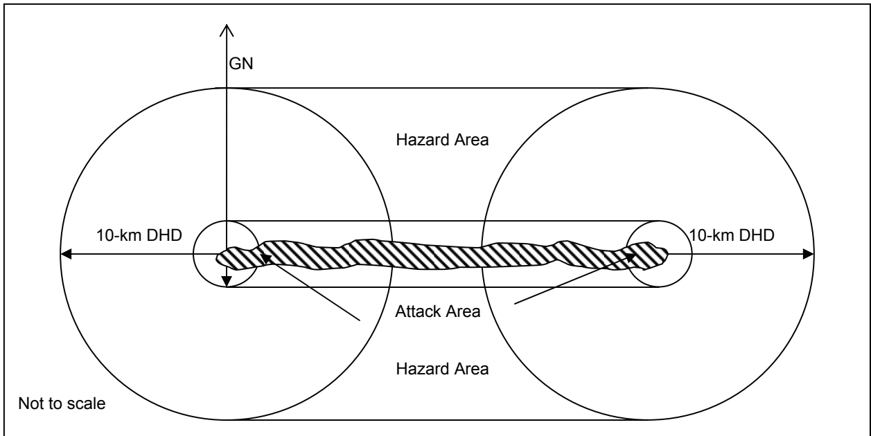
Figure E-11. Hazard Area From Type B, Case 5 (Any Dimension of Attack Area >2 km, Wind Speed ≤10 kph)
