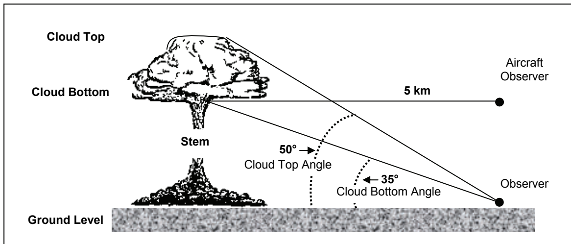
Figure G-5. Stabilized Cloud Top and Cloud Bottom Angle and Height Measurements
