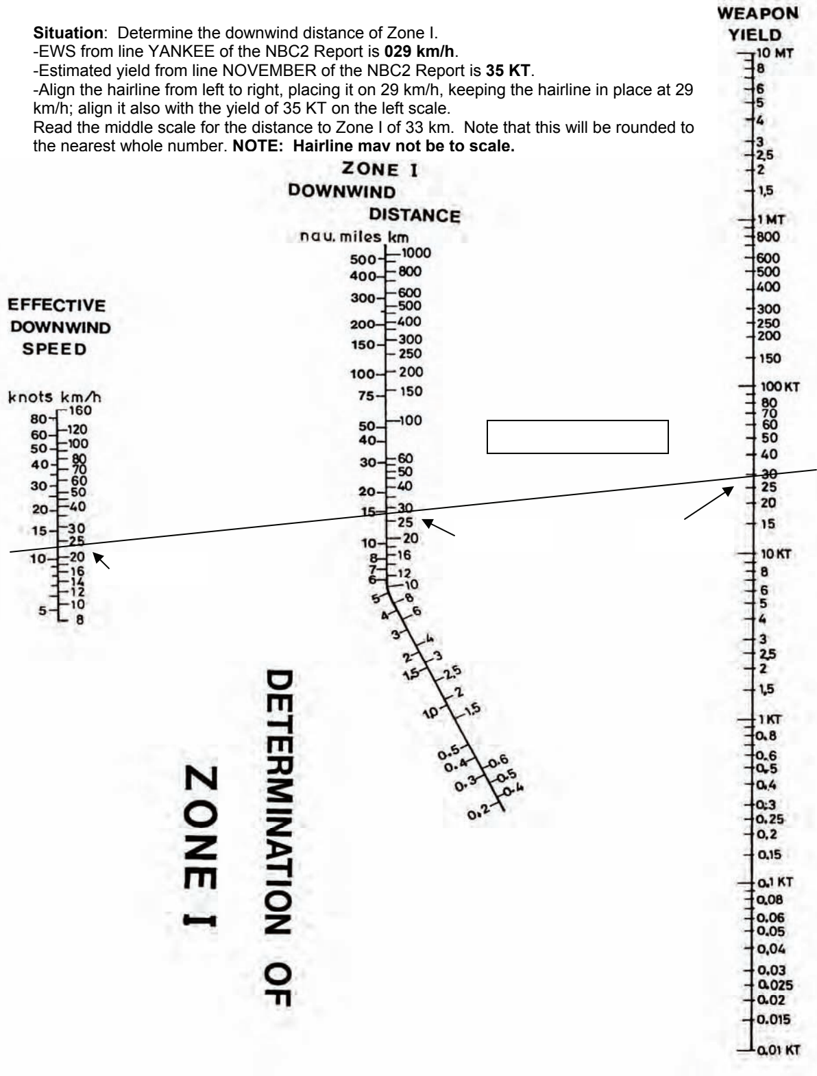
Figure G-16. Determination of Zone I, Downwind Distance (Example)
