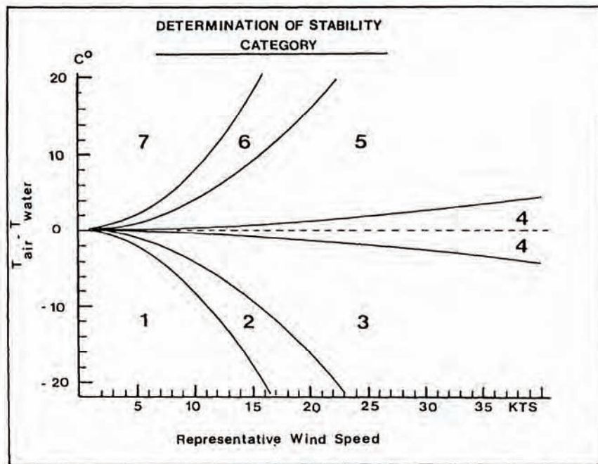
Figure E-21. Air Stability Category (Sea)
