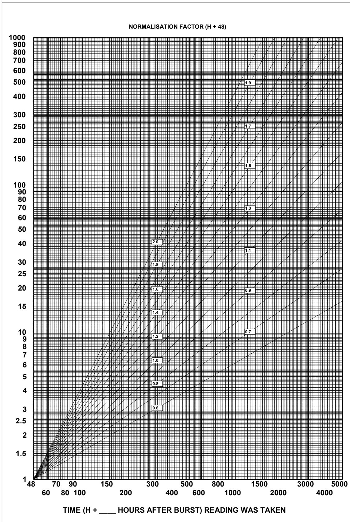
Figure J-48. Graphical Method for Determining Normalization Factor (H+48)
