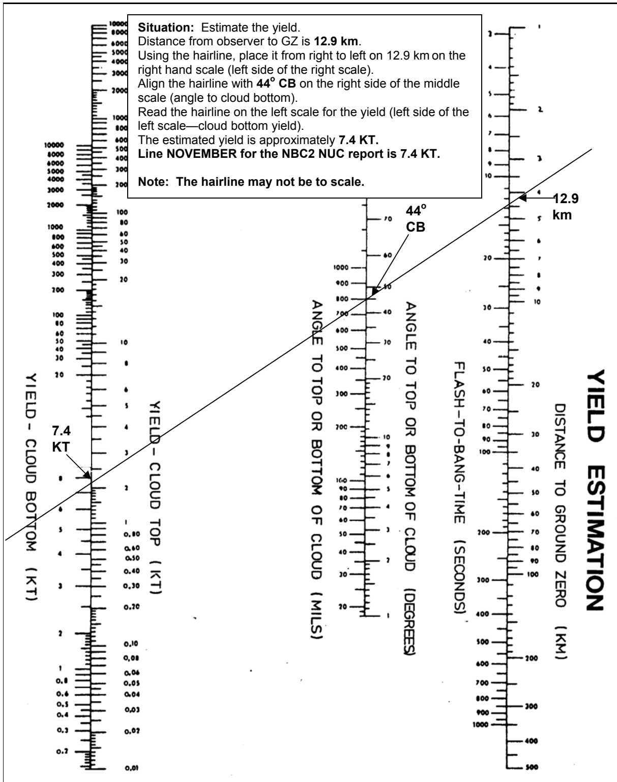
Figure G-10. Yield Estimation, Angle to Top/Bottom of Cloud and Flash-to-Bang Time/Distance to GZ (Example)
