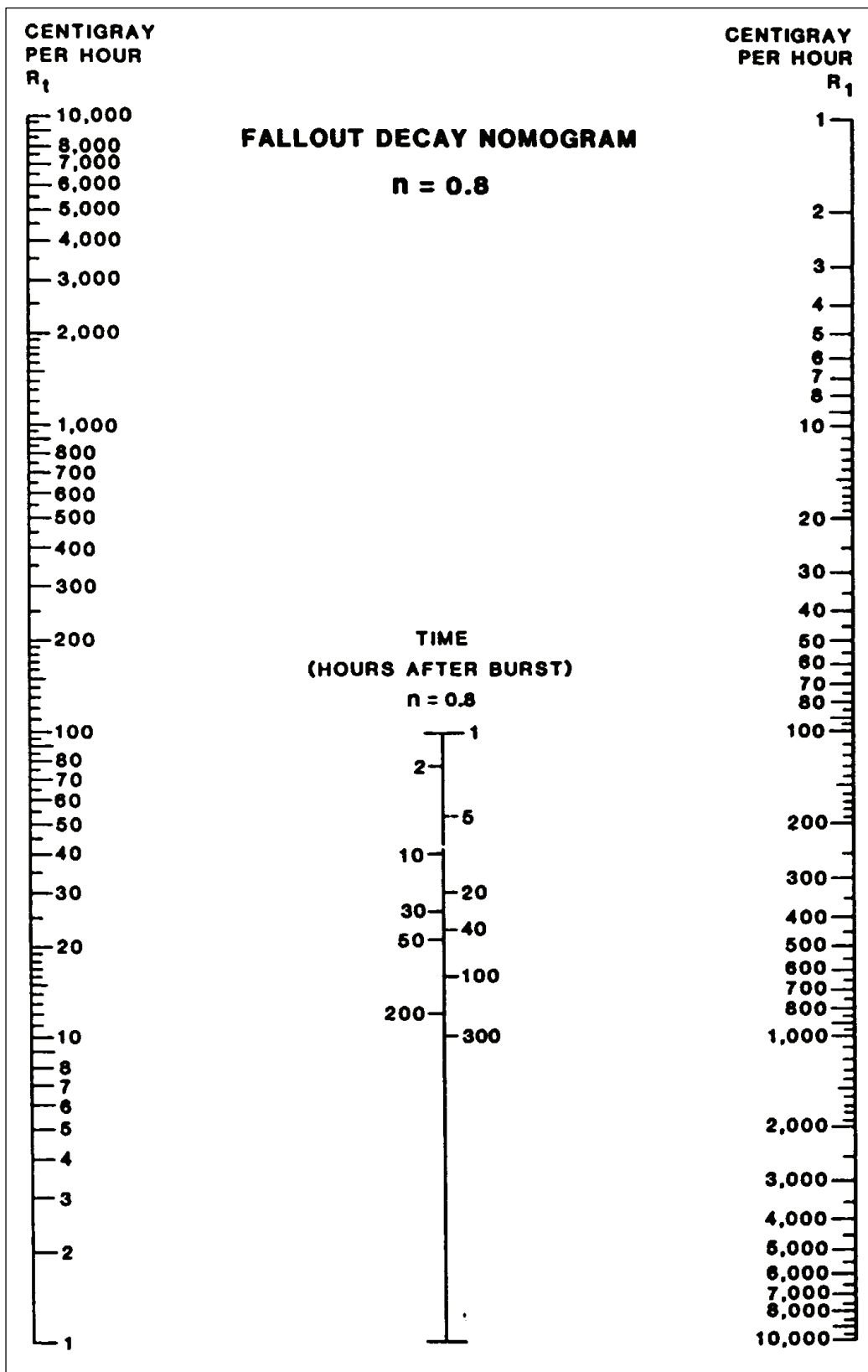
Figure J-15. Fallout Decay Nomogram (n=0.8)
