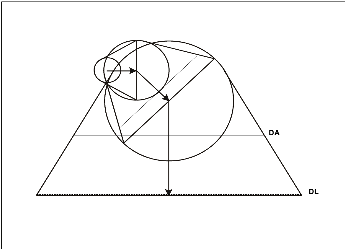
Figure F-12. Type Q, Case 2, Attack (1 Hour Into CDR, Changing Downwind Direction)
