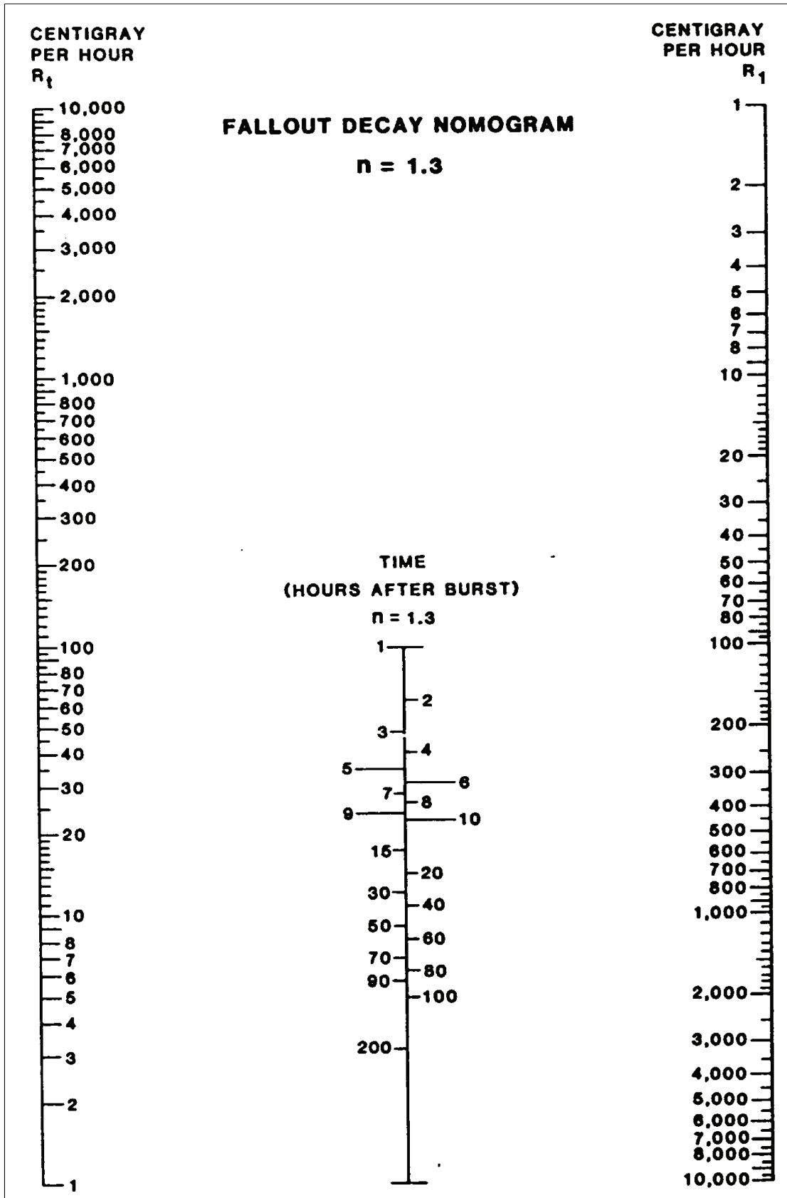
Figure J-20. Fallout Decay Nomogram (n=1.3)
