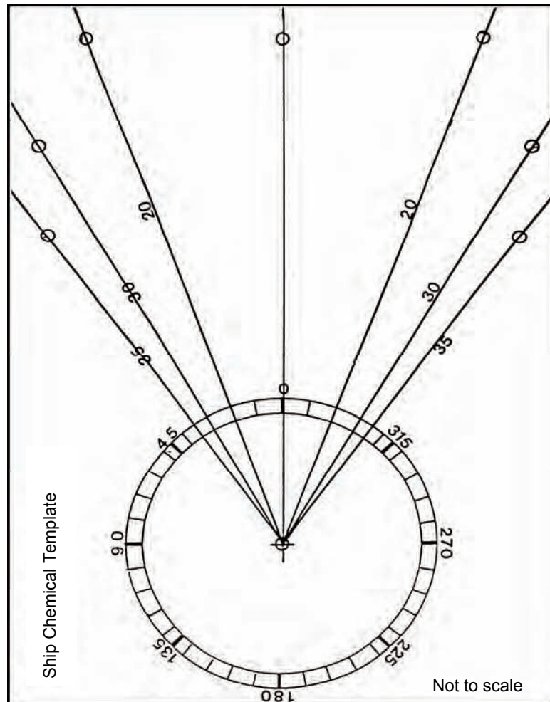
Figure E-22. Ship Chemical Template (Example)
