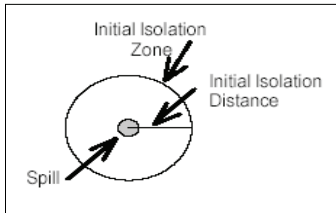
Figure H-6. Type T, Case 5
