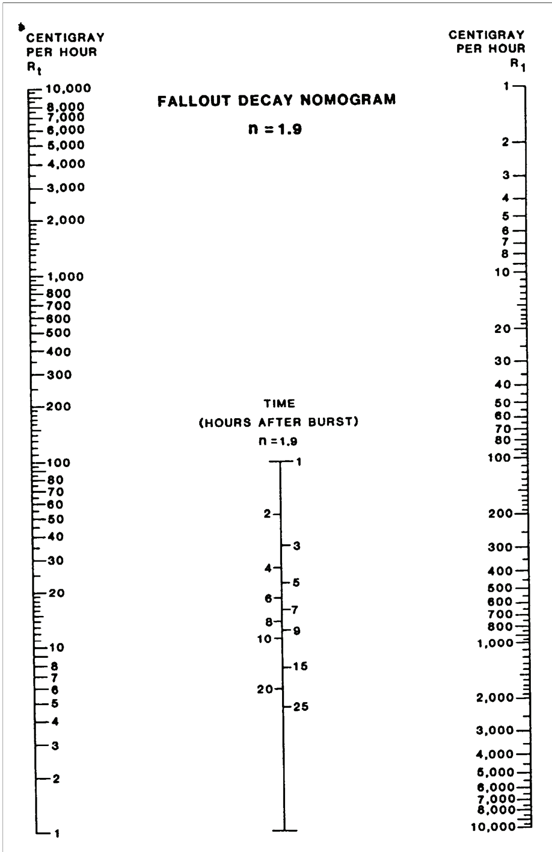
Figure J-26. Fallout Decay Nomogram (n=1.9)
