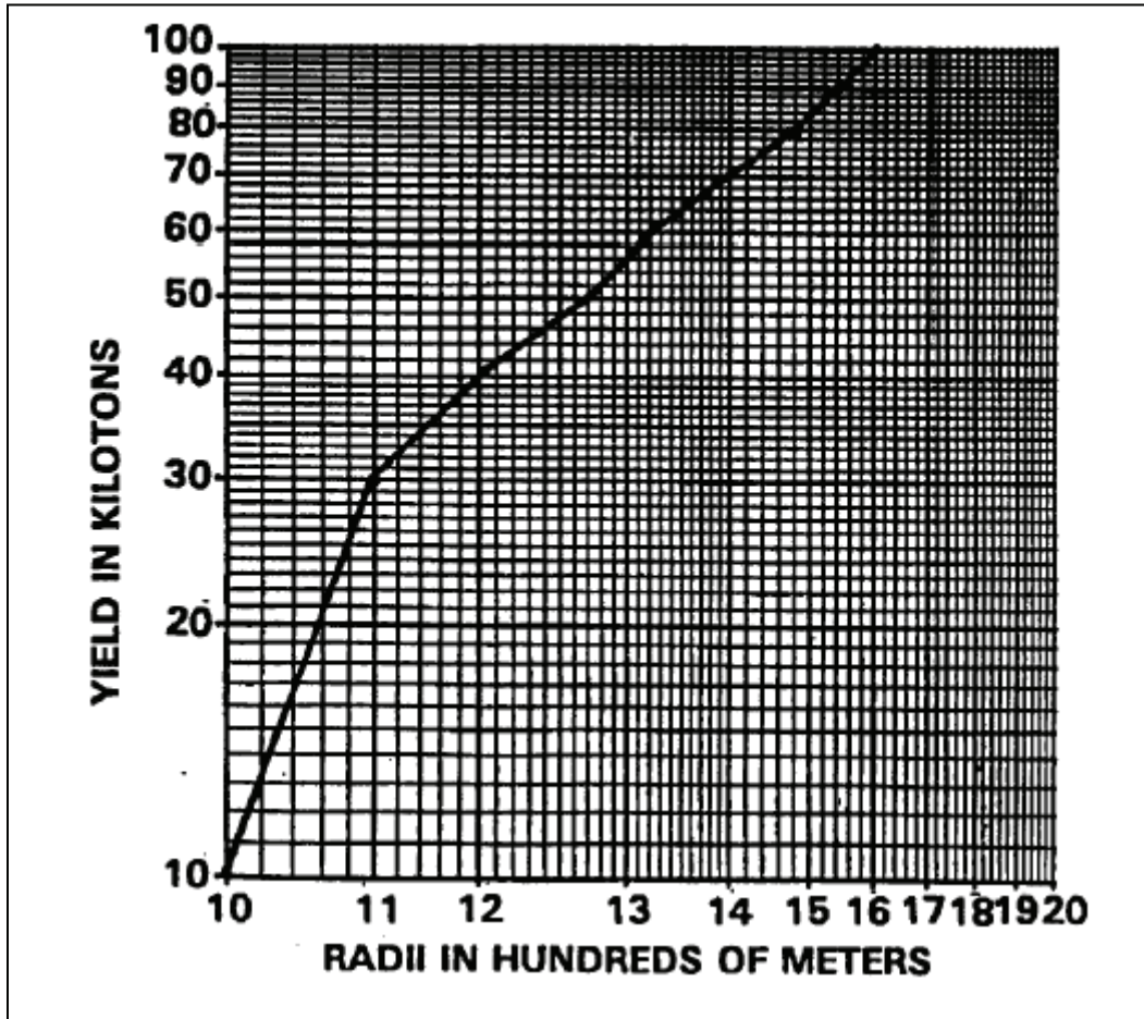
Figure G-38. Keller Nomogram for Neutron-Induced Areas From 10 to 100 Kilotons
