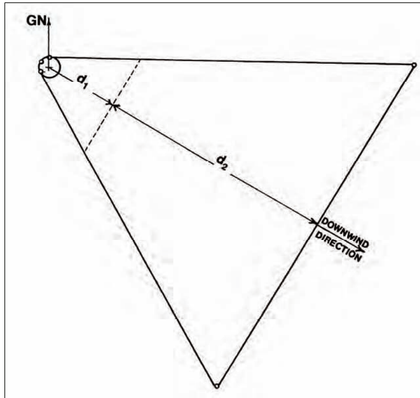
Figure E-19. Recalculation of Downwind Hazard Area Type A, Case 2 Attack (Change in Stability Category and/or Downwind Speed)
