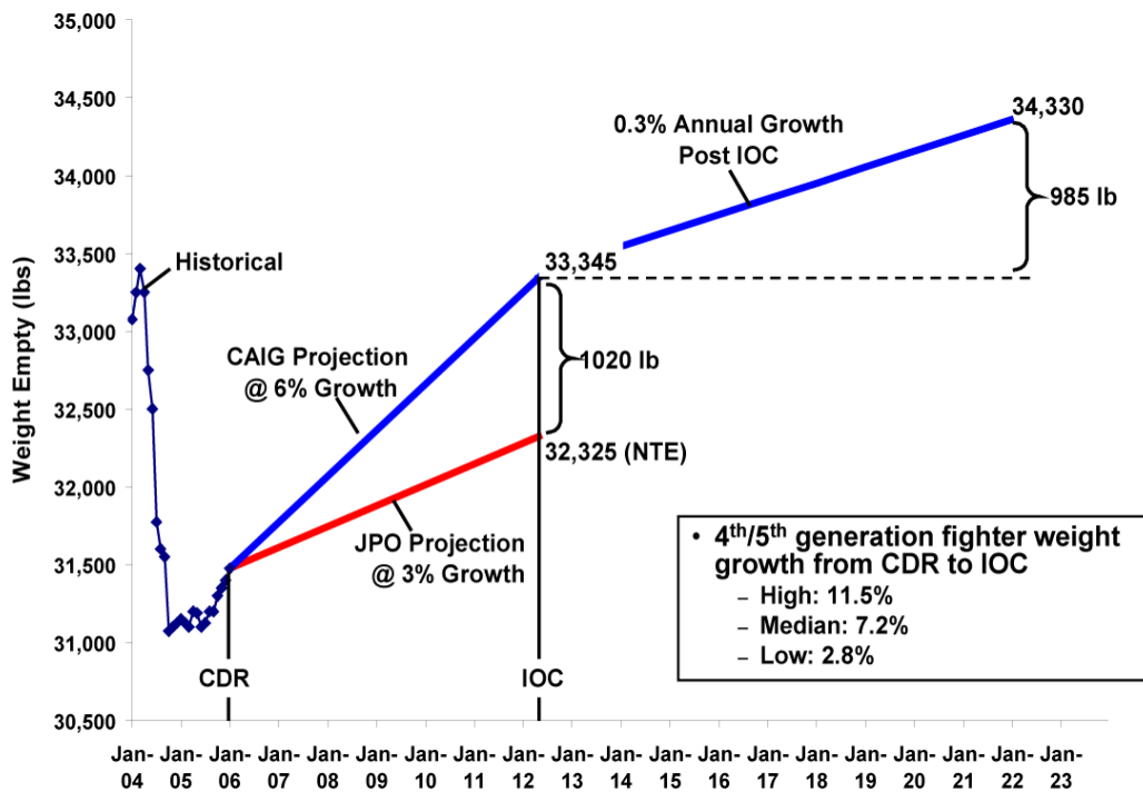
Figure 1. F-35 STOVL Variant Weight Growth Projection
