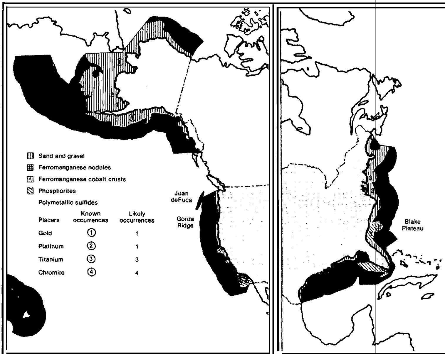
Figure 1-3.—Potential Hard Mineral Resources in the EEZ of the Continental United States, Alaska, and Hawaii
