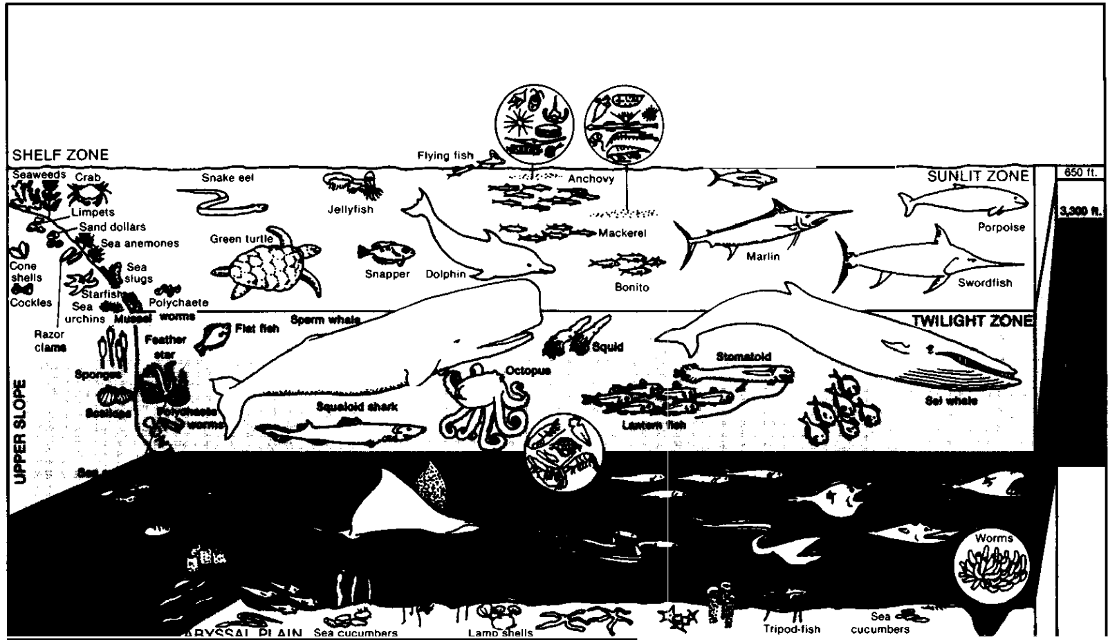
Figure 6-1.—The Vertical Distribution of Life in the Sea
