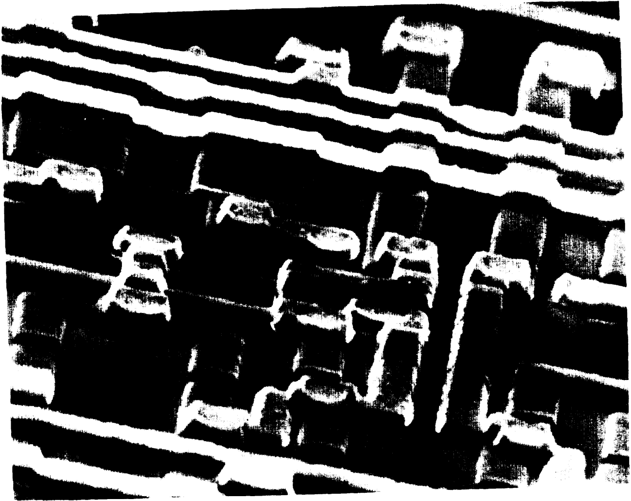
Scanning electron micrograph of a portion of a programmable logic array with locations for up to 4,000 logic elements. The array was fabricated with the one-micrometer FET technology. Reducing the minimum device dimensions to one micrometer resulted in an increase in speed of a factor of 3 or 4, and a reduction in power dissipation by a factor of 10, as compared with previous FET circuits
