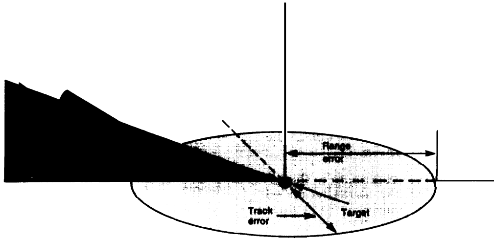
Figure 83.—Down Range and Cross Range Errors of a Ballistic Reentry Vehicle at a Target
